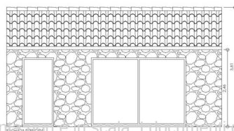
FACHADA PRINCIPAL
