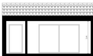
SECTION D-D:
